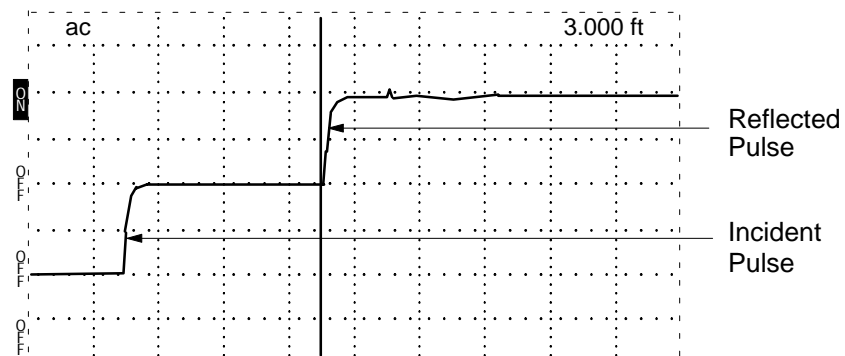
Figure 2-2: Cursor of Rising Edge of Reflected Pulse
