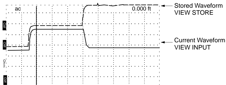
Figure 2-26: Waveform with Both Current and Stored Waveforms
