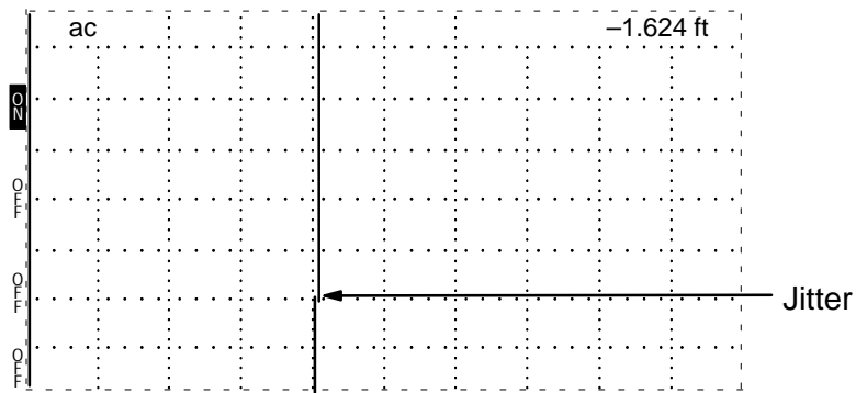
Figure B-16: Jitter Apparent on Leading Edge of Incident Pulse
