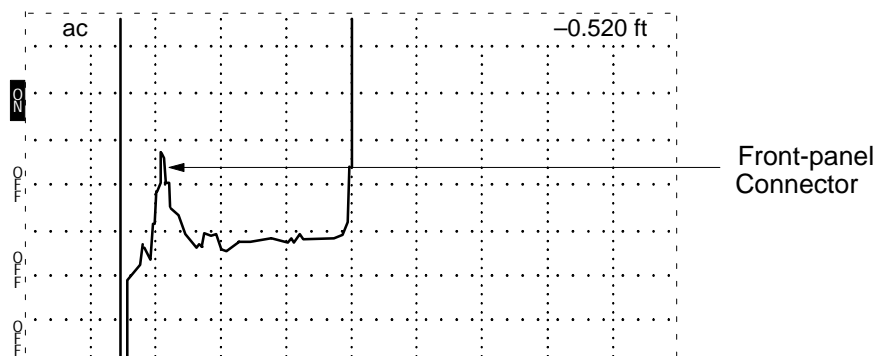
Figure 2-7: 3-foot Cable with Cursor at Incident Pulse, Vertical Scale at 25 dB
