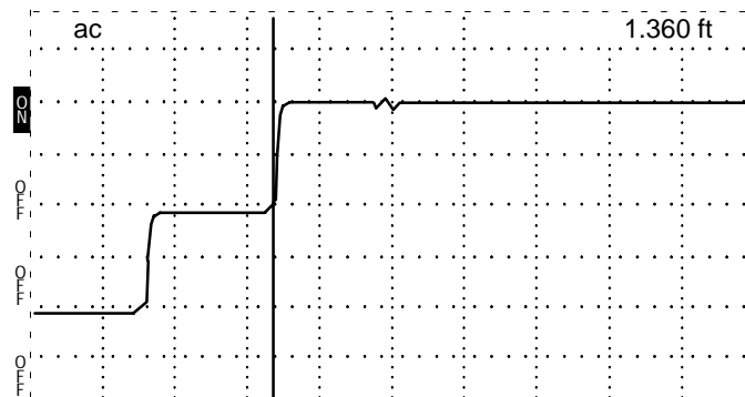
Figure B-4: Cursor at End of 3-foot Cable, V_p Set to .30
