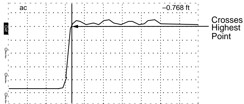
Figure B-15: Cursor on Highest Major Graticule that Rising Edge crosses
