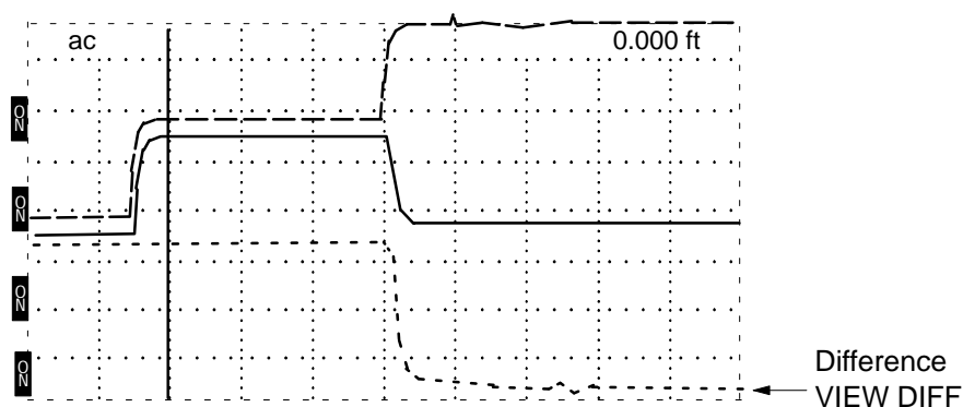
Figure 2-27: Stored, Current, and Difference Waveforms
