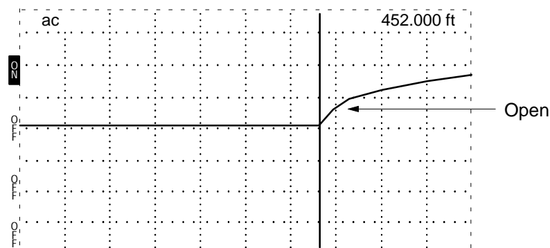
Figure 1–11: 455-ft Cable
